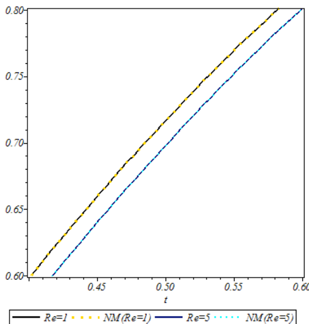
Figure II Effect of Reynolds number on axial velocity
