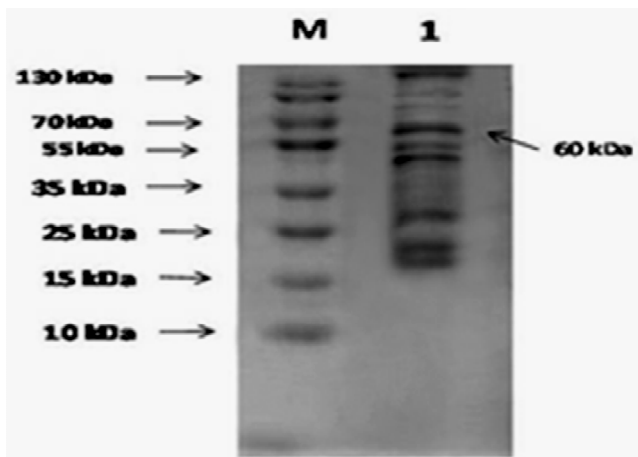
Figure I: SDS-PAGE analysis of purified flagellar antigen (FLA) Lane 1 = Purified FLA antigen, Lane M= Prestained protein ladder
